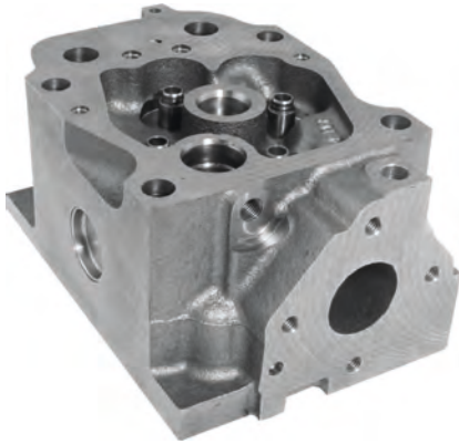
ÜRÜN ADI : SİLİNDİR KAPAĞI BOŞ PRODUCT NAME : CYLINDER HEAD (BLANK) ARAÇ ADI : MERCEDES 1840 EURO 5 VEHICLE ORJ. REF. NO : 457 010 0721 ORJ. REF. NO ÜRÜN NO : C45702001 PRODUCT NO
